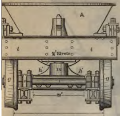
END ELEVATION. FRONT POT REMOVED.
